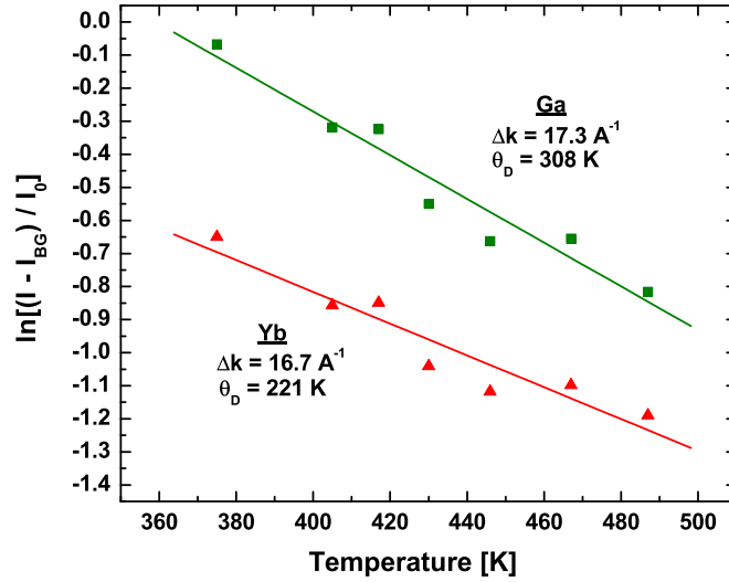
Figure 27. Logarithm of the core peak photoemission intensities for Yb and Ga as a function of temperature following background ( I_{BG} ) subtraction and normalization to the peak intensity at the lowest temperature I_0 . The experimental values were fitted (solid line) with the Debye-Waller factor.
