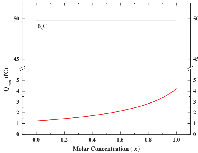
Figure 39. Q_{max} creation from (red): a single ^{157}Gd neutron capture event resulting in 79 keV internal conversion electron emission, as a function of molar concentration x in Gd_xGa_{1-x}N ; (black): a single neutron capture event in B_5C resulting in 0.84 MeV ^7Li ion production, as shown in (88).
