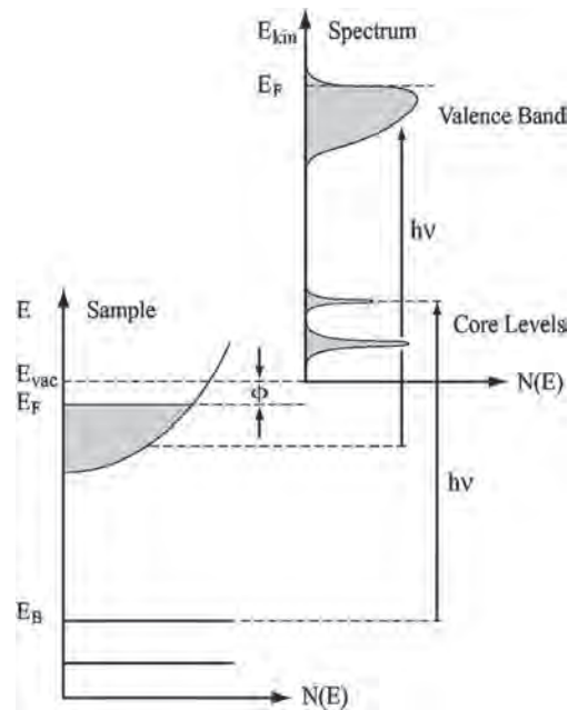
Figure 7. The photoelectron energy distribution produced by incoming photons and measured as a function of the kinetic energy E_{kin} of the photoelectrons (right) is more conveniently expressed in terms of the binding energy E_B (left) when one refers to the density of states inside the solid ( E_B = 0 at E_F .) Adapted from [1].
